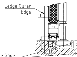
e) Flat Steel Threshold S10D
