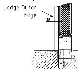
d) Thresholdless Latch Stop RA
