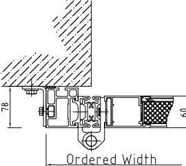
a) In front of or behind the reveal IR/BR
