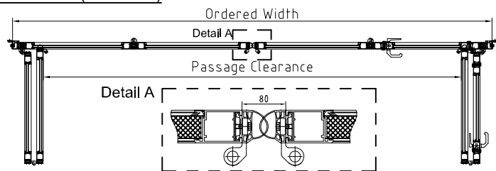
Assembly Situation (Scale 1:10)
