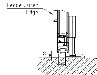
b) Flat steel Threshold S20D
