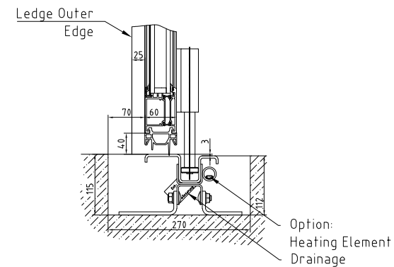
c) Floorguide -light Niro
