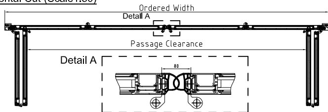
Horizontal Cut (Scale1:50)
